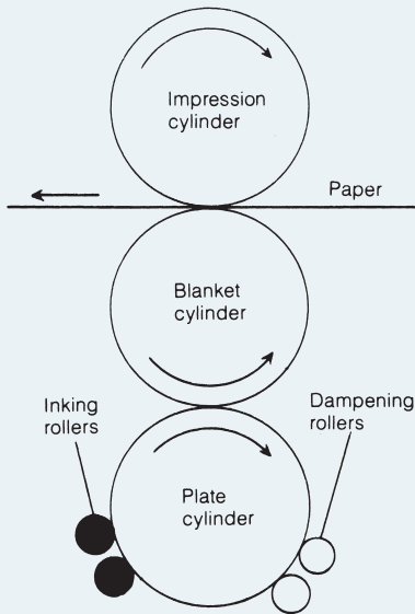
Fig. A.10. Principle of offset printing. A plate is wrapped around and fastened to the plate cylinder. Water applied by the dampening rollers adheres only to the background area of the plate; ink applied by the inking rollers adheres only to the dry image of the type on the plate. As the plate cylinder revolves, it transfers the ink to the rubber blanket of the blanket cylinder, which in turn transfers (or offsets) it onto the paper, which is held in place by the impression cylinder.
